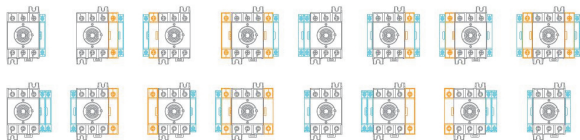
Figure 30 Schematic diagram of accessory pole/auxiliary contact matching
