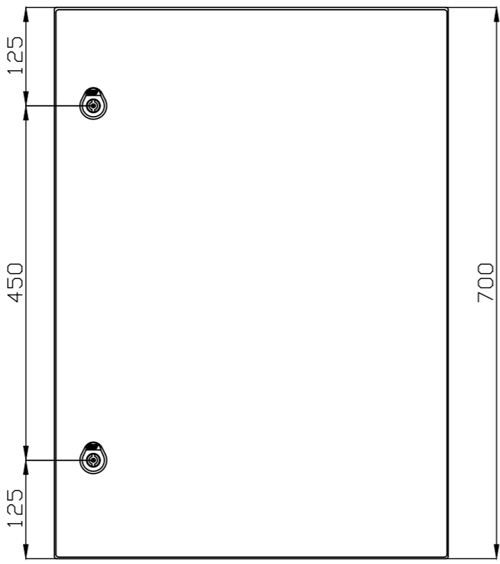
GN705030
