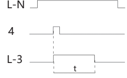
type H delay time sequence chart
