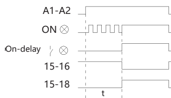
type Di delay time sequence chart
