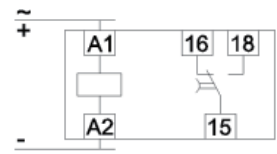
NTE8-M2 wiring diagram
