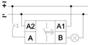
NTE8-C (3 wires) wiring diagram
