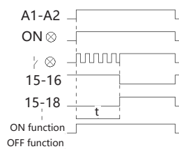
type W delay time sequence chart
