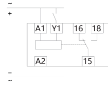
NTE8-M2 wiring diagram
