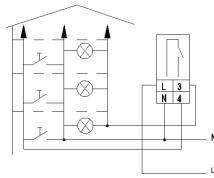
NTE8-C (3 wires) wiring diagram
