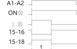
type A delay time sequence chart
