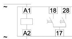
NTE8-Y wiring diagram
