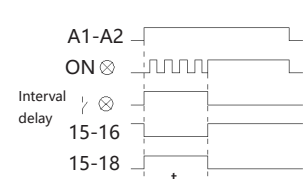
type H delay time sequence chart
