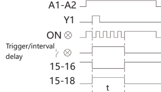
type B delay time sequence chart
