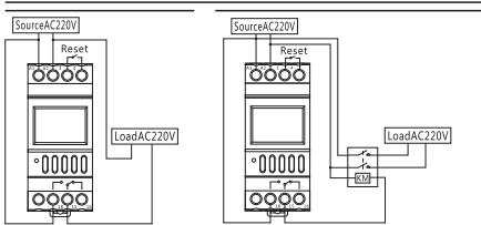
Figure 2 Wiring method of single phase control
