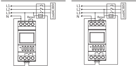
Figure 4 Wiring diagram of 3-phase control (contactor coil AC220V)
