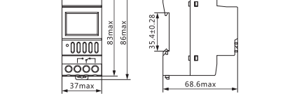
Figure 1 Outline and installation dimensions
